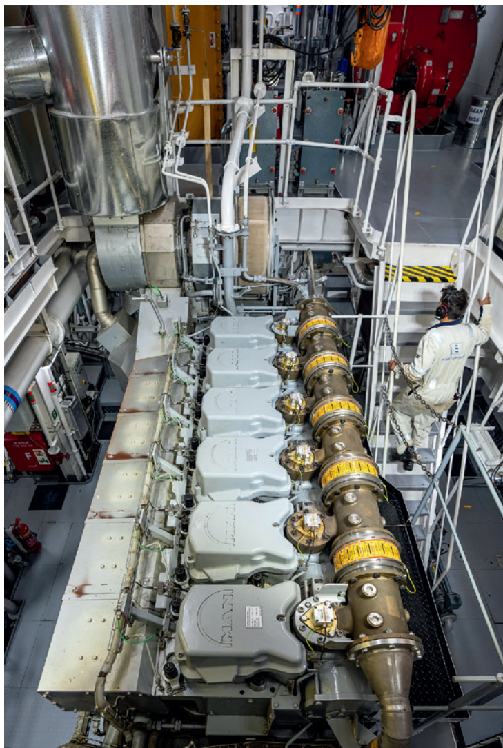
Impressive 4,325 hp dual-fuel MAN main engine with LNG pipeline
